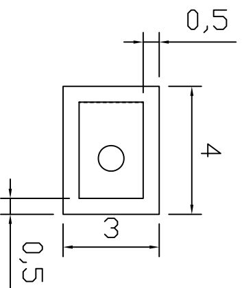
PCB Layout Recommendation
