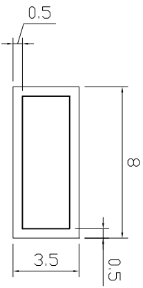
PCB Layout Recommend
