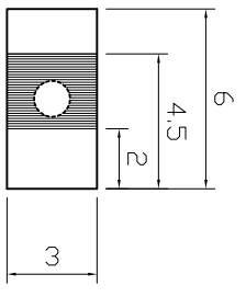
SOLDER PAD DIMENSION
