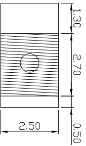
PAD DIMENSION RECOMMEND
