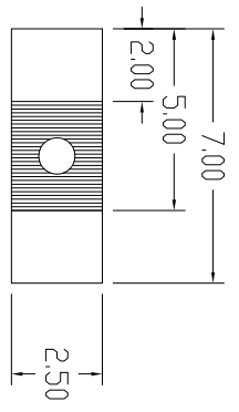
SOLDER PAD DIMENSION
