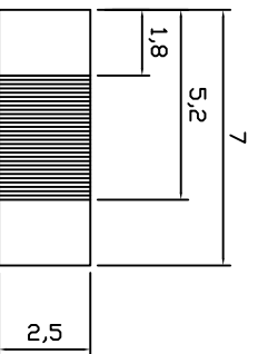
SOLDER PAD DIMENSION
