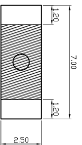
SOLDER PAD DIMENSION
