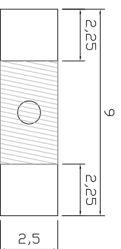
SOLDER PAD DIMENSION
