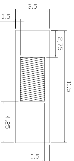
PCB Layout Recommend
